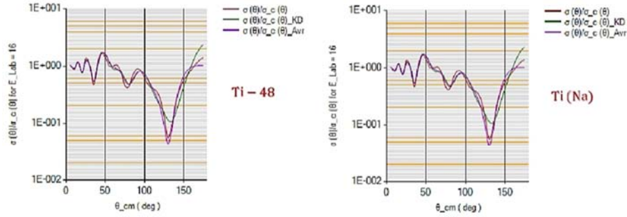
Figure 8. Dependence of the (\alpha + {}^{48,natural}\text{Ti}) (\sigma_c/\sigma) ratio upon the center-of-mass scattering angle (the red line) compared with these resulted from global parametrization of the optical model potential, for E_{\text{Lab}} = 16 MeV.
