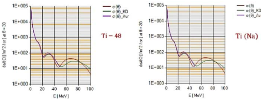
Figure 11. The energy dependence of the (\alpha + {}^{48,natural}\text{Ti}) elastic differential cross section (the red line) compared with these resulted from global parametrization of the optical model potential, for \theta_{\text{cm}} = 30^\circ .
