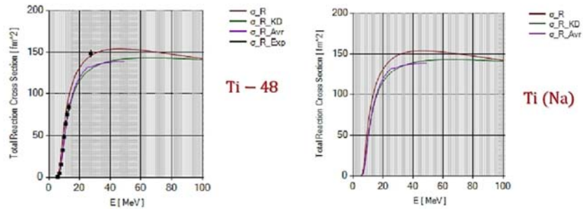
Figure 5. The energy dependence of the ( \alpha + {}^{48,natural}\text{Ti} ) total reaction cross section (the red line) compared with experimental values and with these resulted from the global parametrization of the optical model potential.
