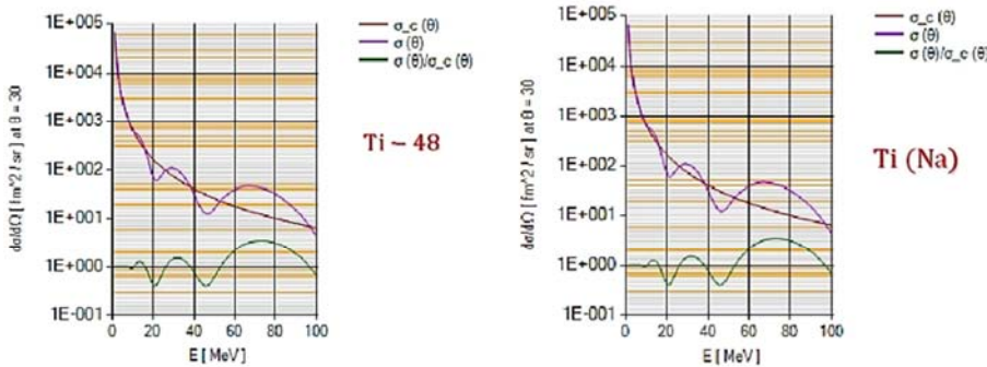
Figure 10. The energy dependence of the (\alpha + {}^{48,natural}\text{Ti}) Coulomb, elastic differential cross sections and (\sigma_c/\sigma) ratio for the center-of-mass scattering angle, \theta_{\text{cm}} = 30^\circ .
