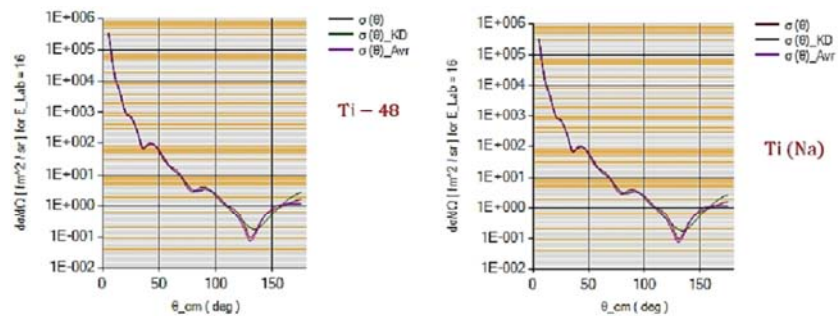
Figure 7. Dependence of the ( \alpha + {}^{48,natural}\text{Ti} ) elastic differential cross section upon the center-of-mass scattering angle (the red line) compared with these resulted from global parametrization of the optical model potential, for E_{Lab} = 16 MeV.
