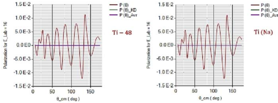
Figure 9. Dependence of the (\alpha + {}^{48,natural}\text{Ti}) polarization upon the center-of-mass scattering angle (the red line) compared with these resulted from global parametrization of the optical model potential, for E_{\text{Lab}} = 16 MeV.
