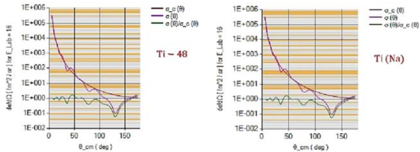
Figure 6. Dependence of the ( \alpha + {}^{48,natural}\text{Ti} ) Coulomb, elastic differential cross sections and ( \sigma_c/\sigma ) ratio upon the center-of-mass scattering angle, for E_{Lab} = 16 MeV.
